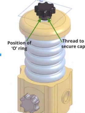
Component A - Water Vessel Cap
