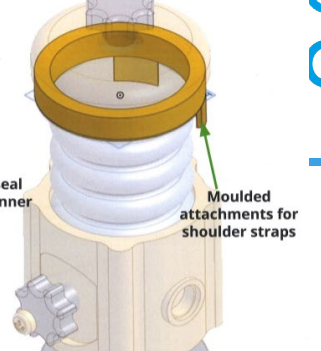
Component C - Lower Lid/Strap Attachment
